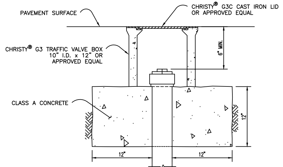
DETAIL B CLEANOUT RISER IN PAVED, TRAFFICKED AREAS
