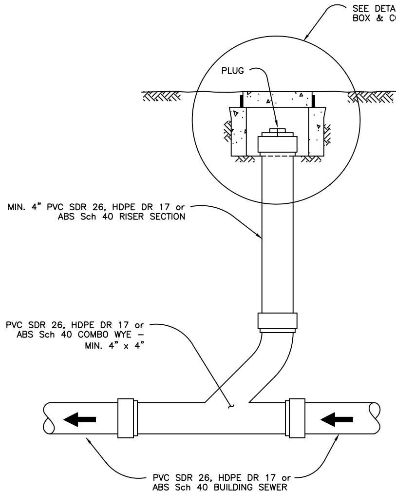
CLEANOUT RISER
