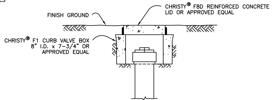
DETAIL A CLEANOUT RISER IN UNPAVED, NON-TRAFFICKED AREAS
